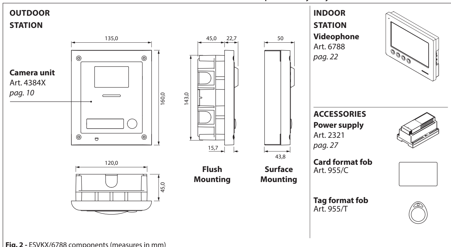
Fig. 2 - ESVKX/6788 components (measures in mm)
