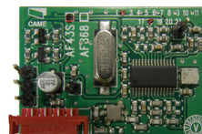
AF435 Plug-in
